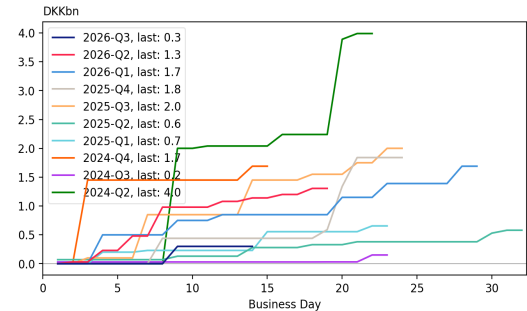
BOLIGX | 1.0 | NDA: Iss. Net of Refi Auctions (OMX)
