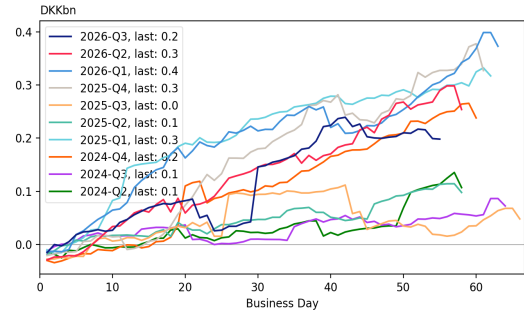
MBB | 30Y IO30 | NDA: Iss. Net of Buybacks and Refi Auctions (CIRMIL)
