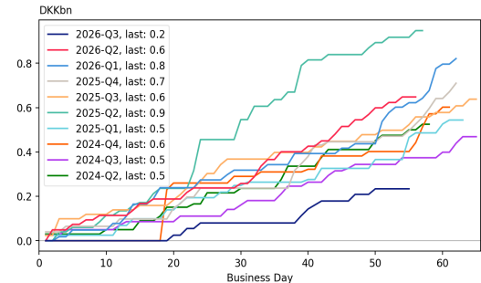
MBB | 30Y A | DLR: Iss. Net of Refi Auctions (OMX)
